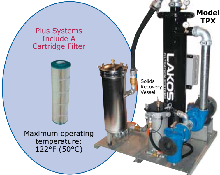
Includes Models TPI and TPX TPX Models are accessible separators
