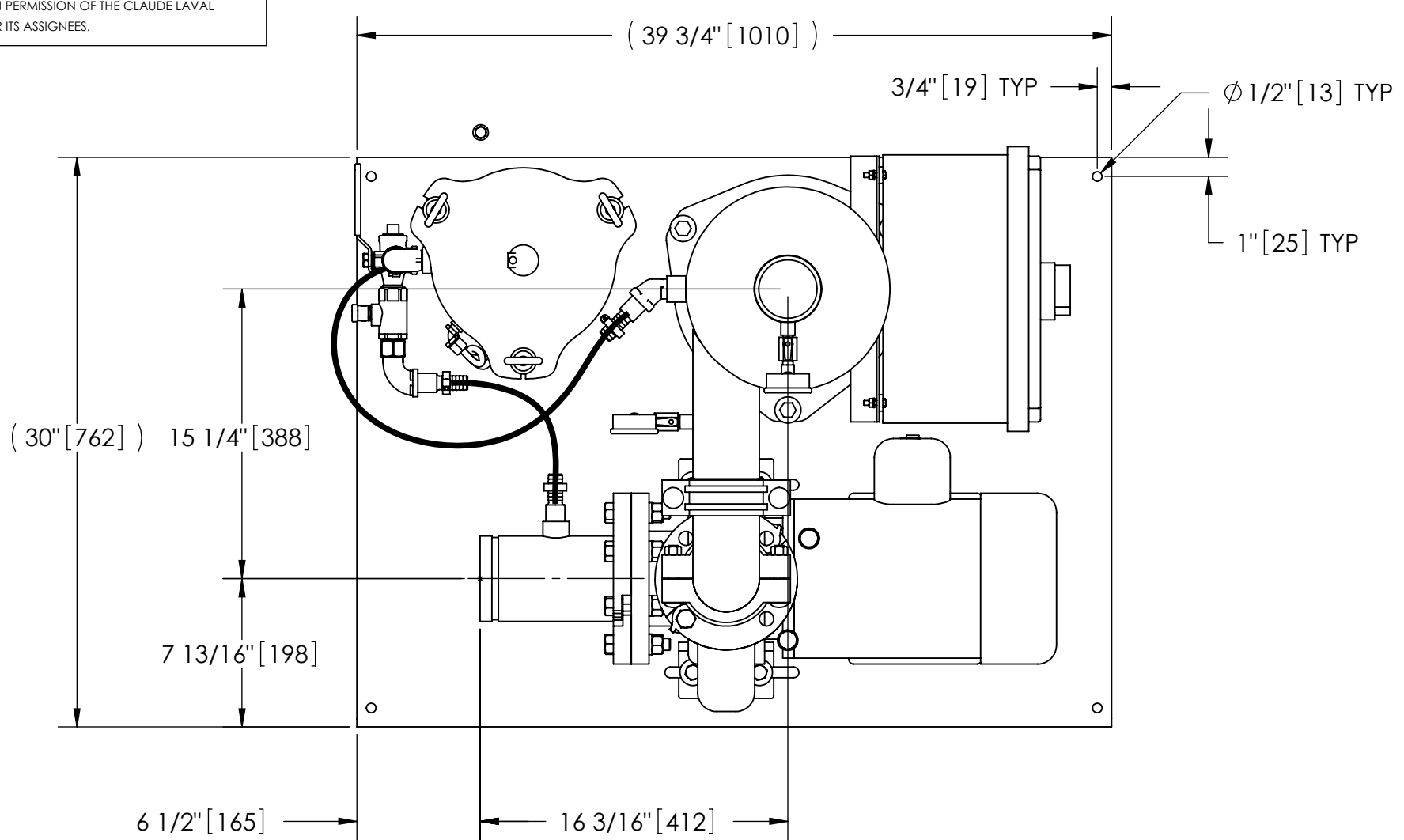
TOP VIEW
