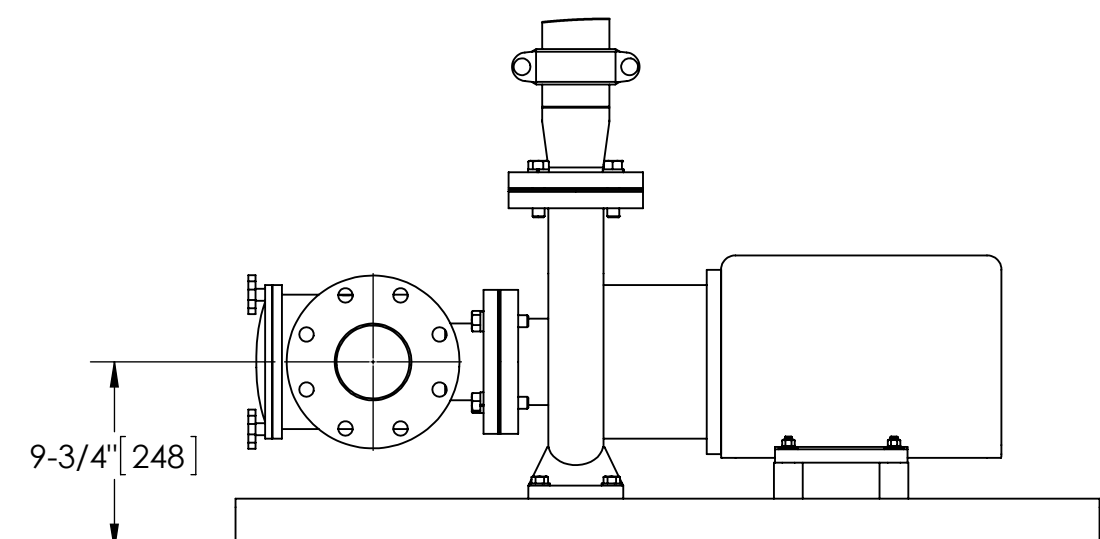
FRONT VIEW ROTATED STRAINER (OPTIONAL)
