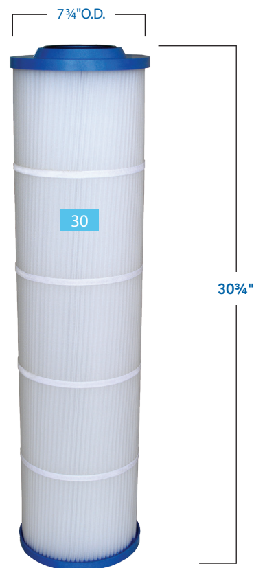
Lakos® Poly-Mesh Cartridges Length and O.D.
