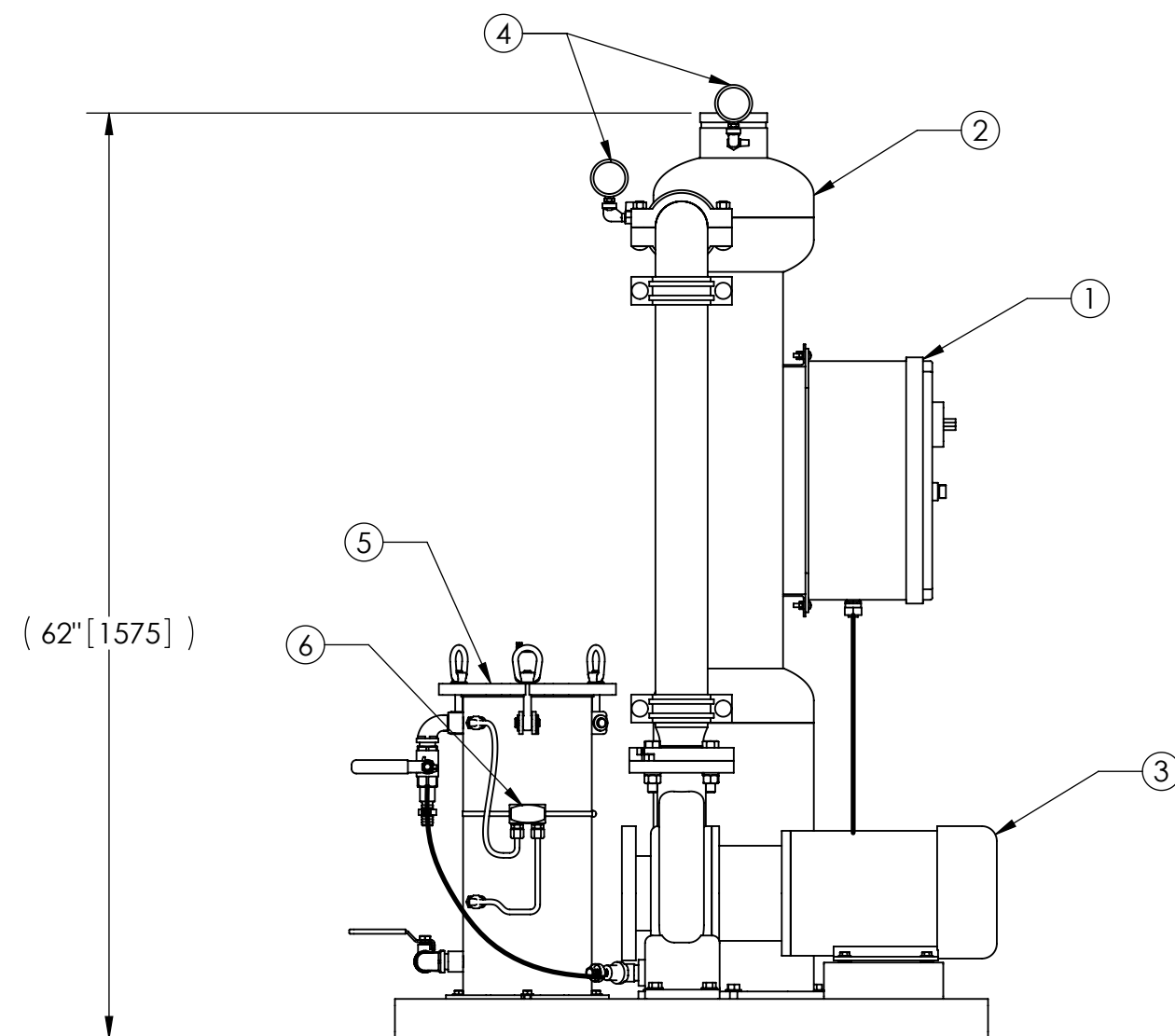
SIDE VIEW W/O TEE
