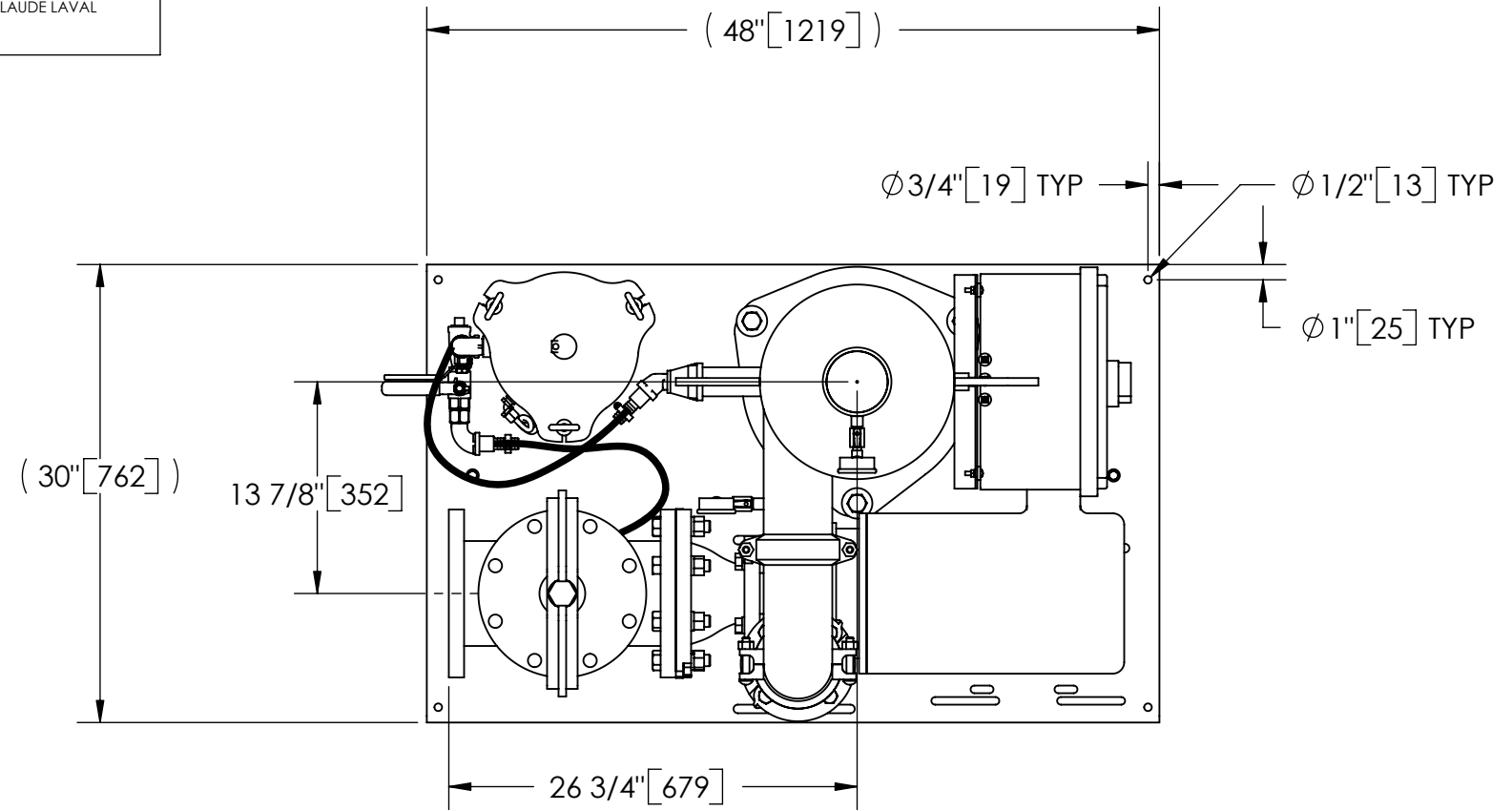
TOP VIEW
