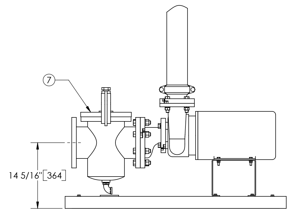
FRONT VIEW PUMP & STRAINER
