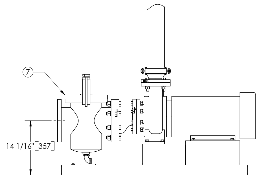
FRONT VIEW PUMP & STRAINER
