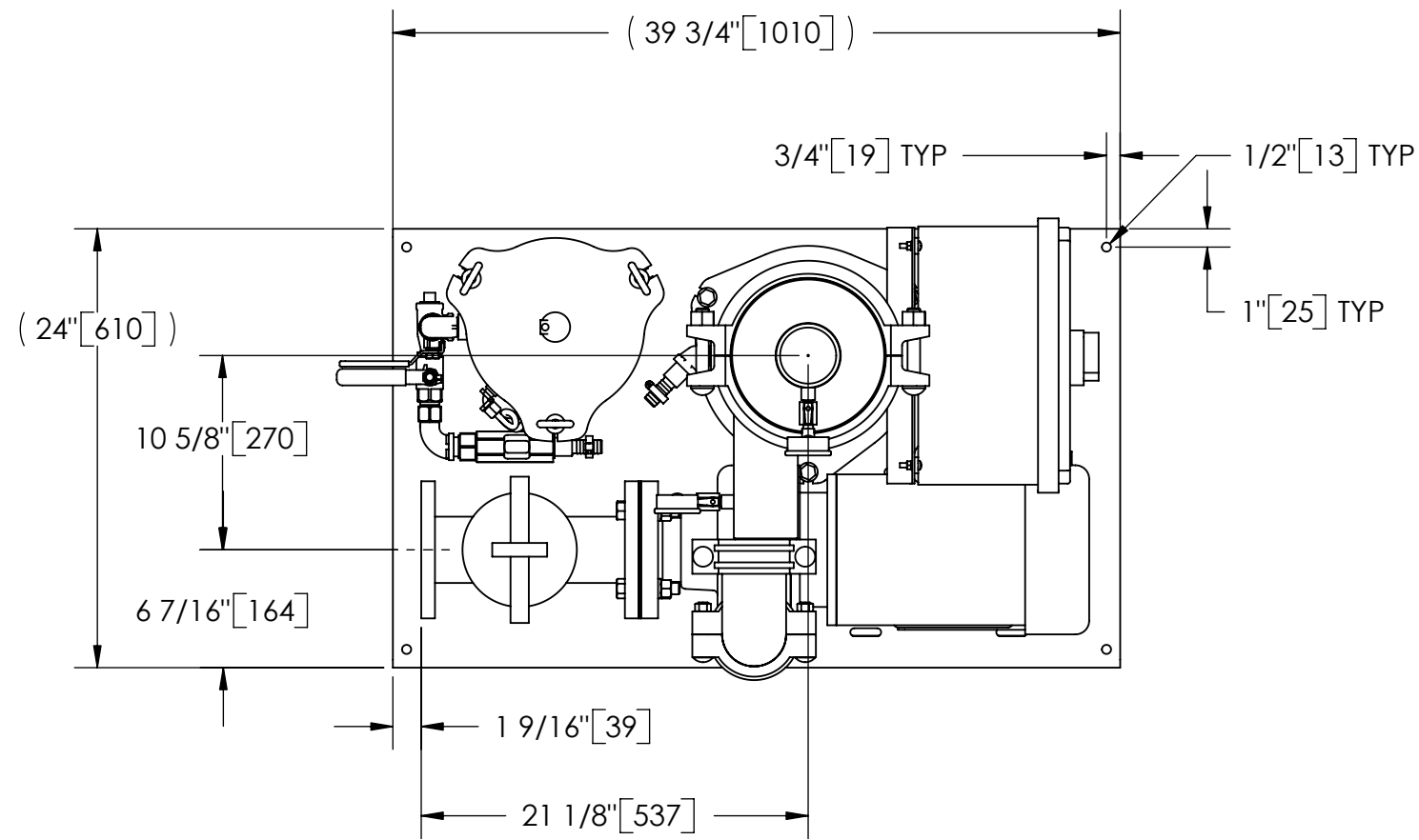
TOP VIEW
