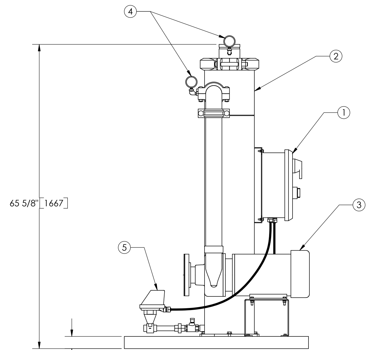
FRONT VIEW W/OUT STRAINER
