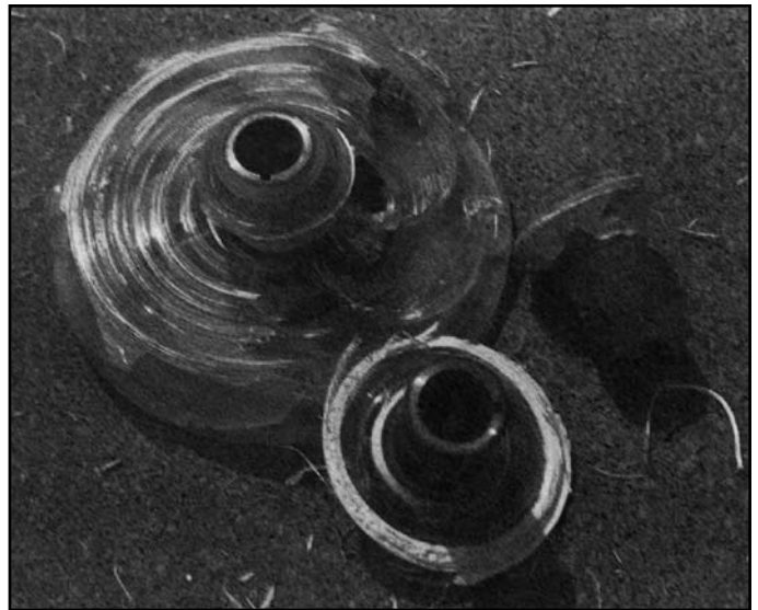
As sand chewed up these impellers, it not only reduced the pump’s performance but also caused the shavings and chips to plug household appliance screens, sprinklers, etc.
