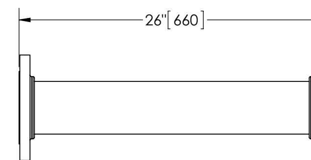
OPTIONAL FLANGED SPOOL MODEL FS-04 (AVAILABLE SEPARATELY) REQUIRED FOR REMOVAL OF TOP ASSEMBLY
