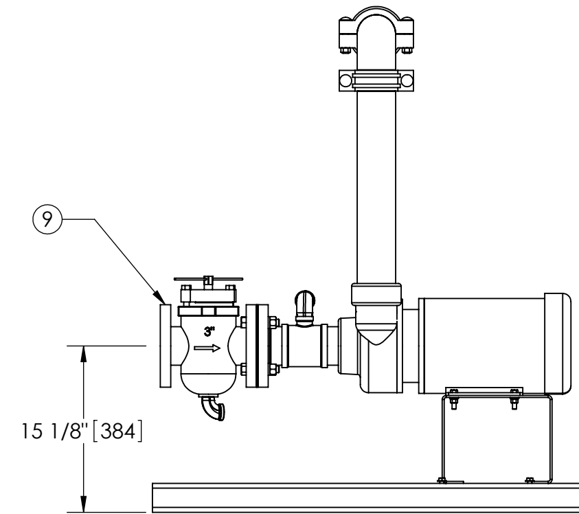
FRONT VIEW PUMP/STRAINER
