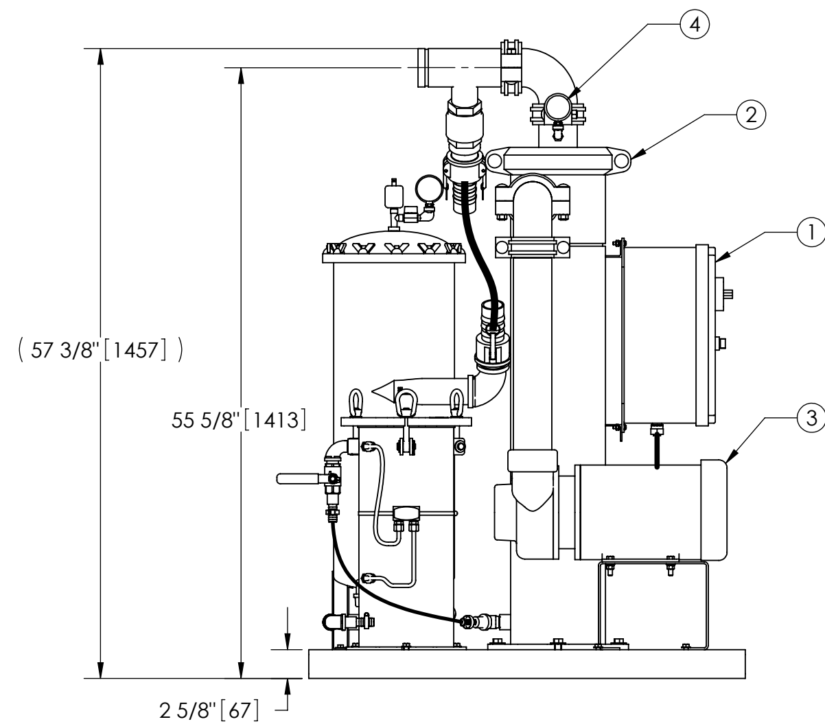
FRONT VIEW W/O STRAINER/SRV
