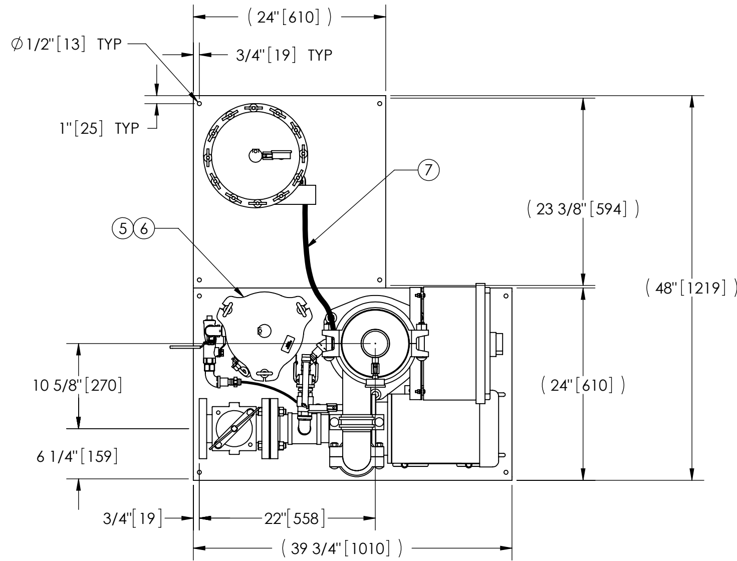
TOP VIEW
