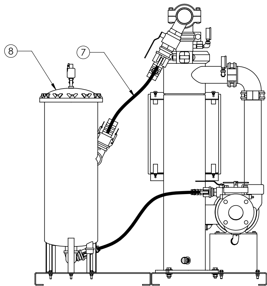
SIDE VIEW W/O SRV
