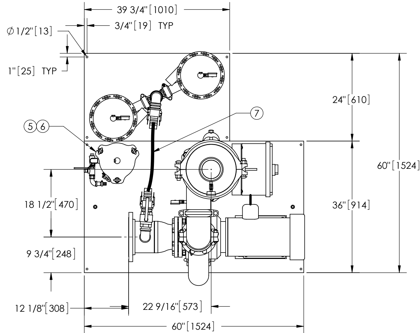
TOP VIEW
