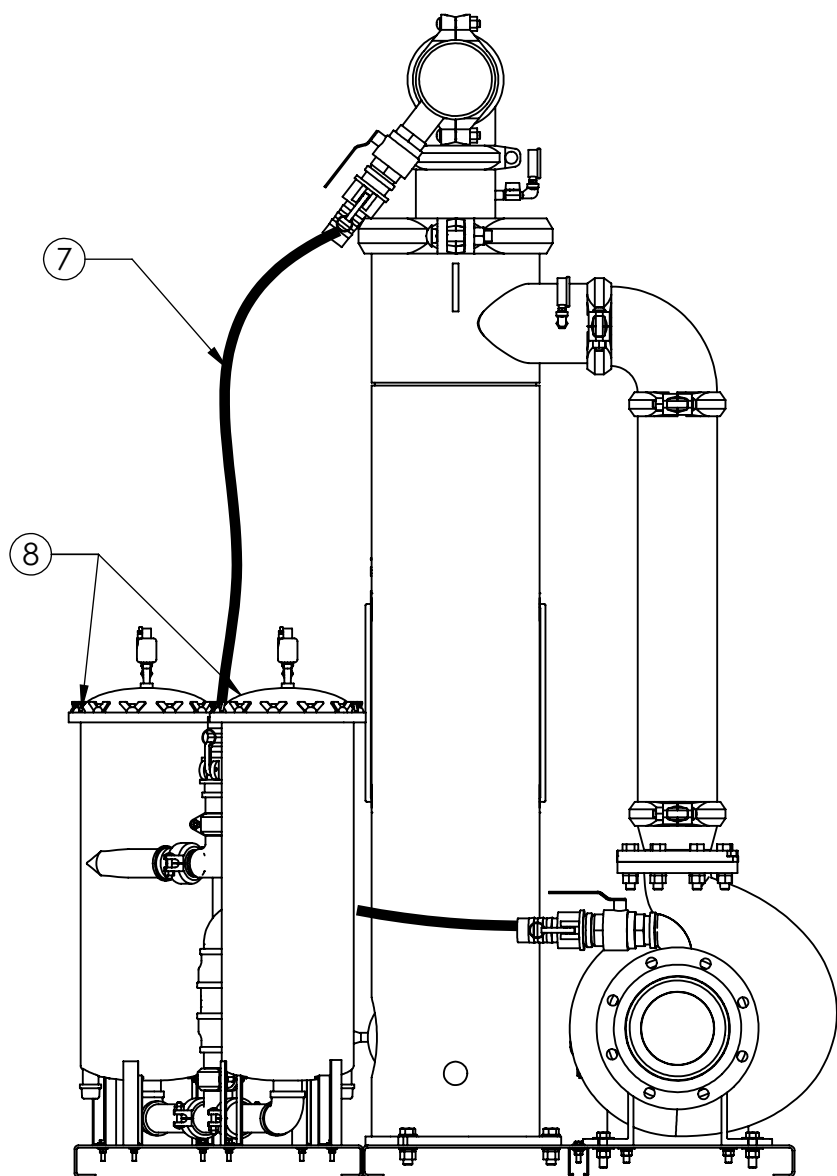
SIDE VIEW W/O SRV
