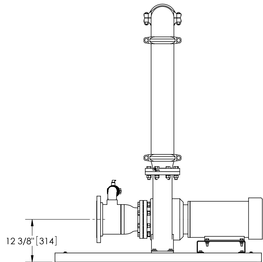
FRONT VIEW PUMP/SPOOL
