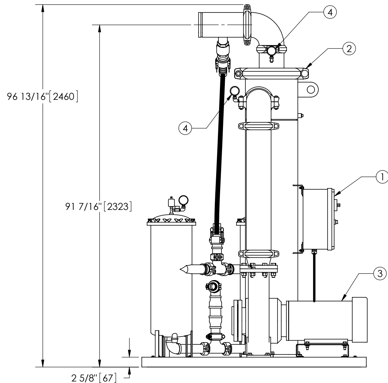
FRONT VIEW W/O SPOOL/SRV
