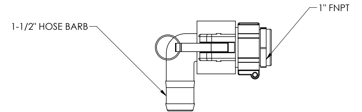
1-1/2" QUICK DISCONNECT ADAPTER (INCLUDED) SCALE 1:3
