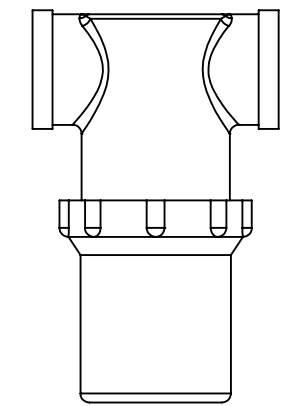
1-1/2" INLINE STRAINER (INCLUDED) 1:4
