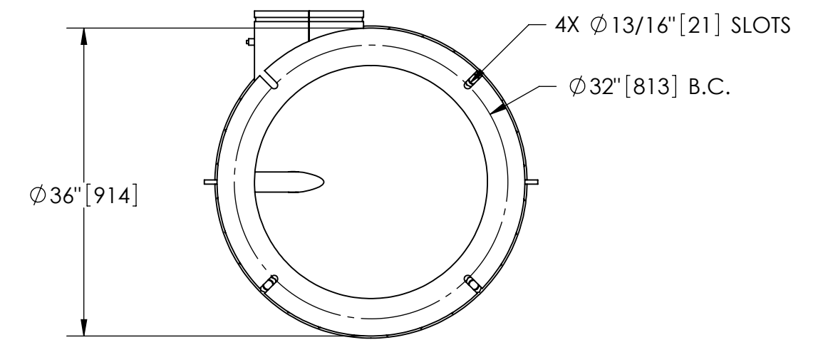
BOTTOM VIEW
