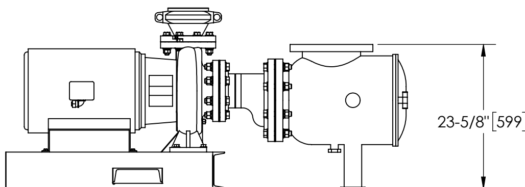
FRONT VIEW PUMP & STRAINER
