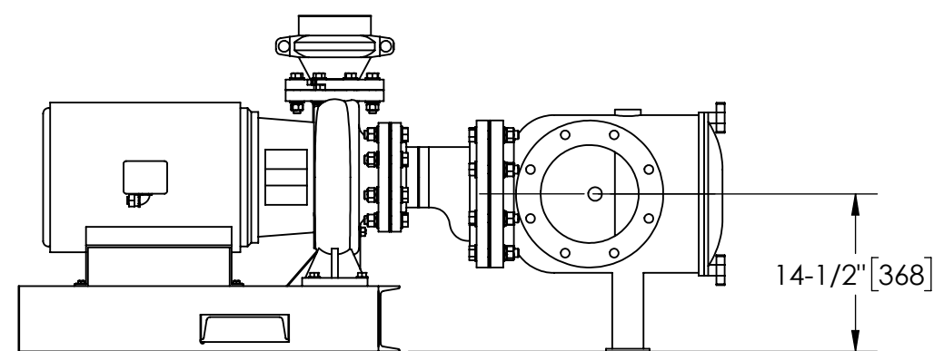
FRONT VIEW ROTATED STRAINER (OPTIONAL)
