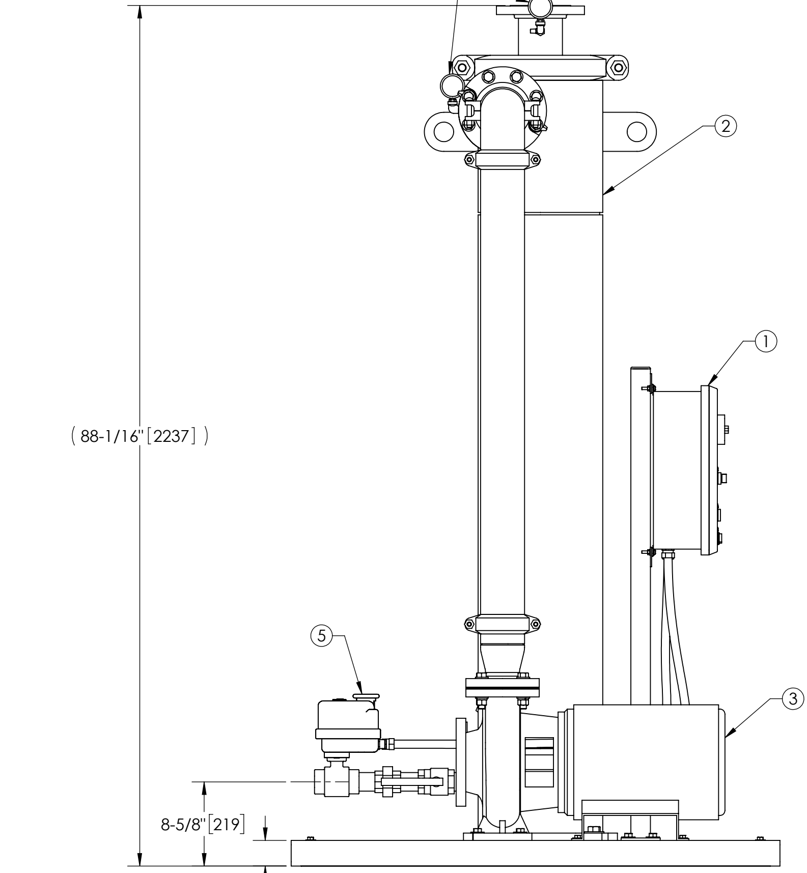
FRONT VIEW W/O STRAINER
