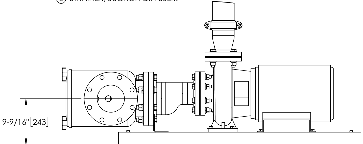
FRONT VIEW ROTATED STRAINER (OPTIONAL)
