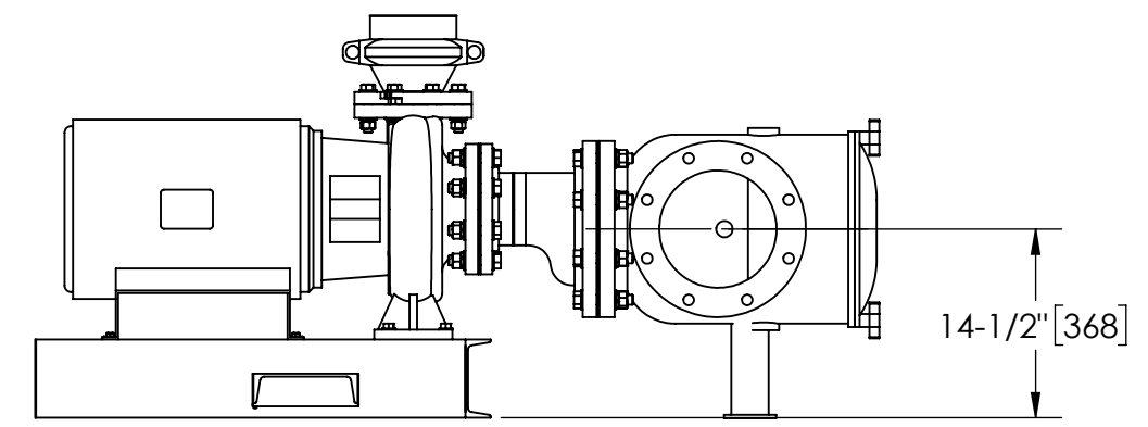
FRONT VIEW ROTATED STRAINER (OPTIONAL)
