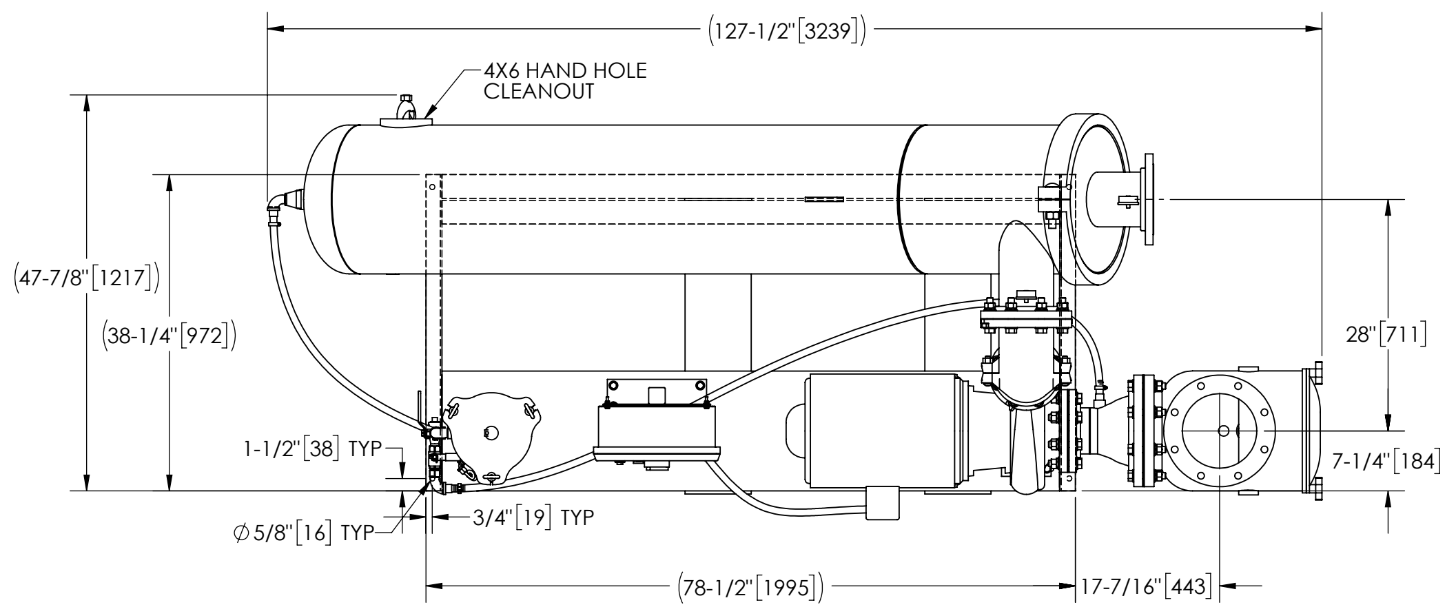
TOP VIEW
