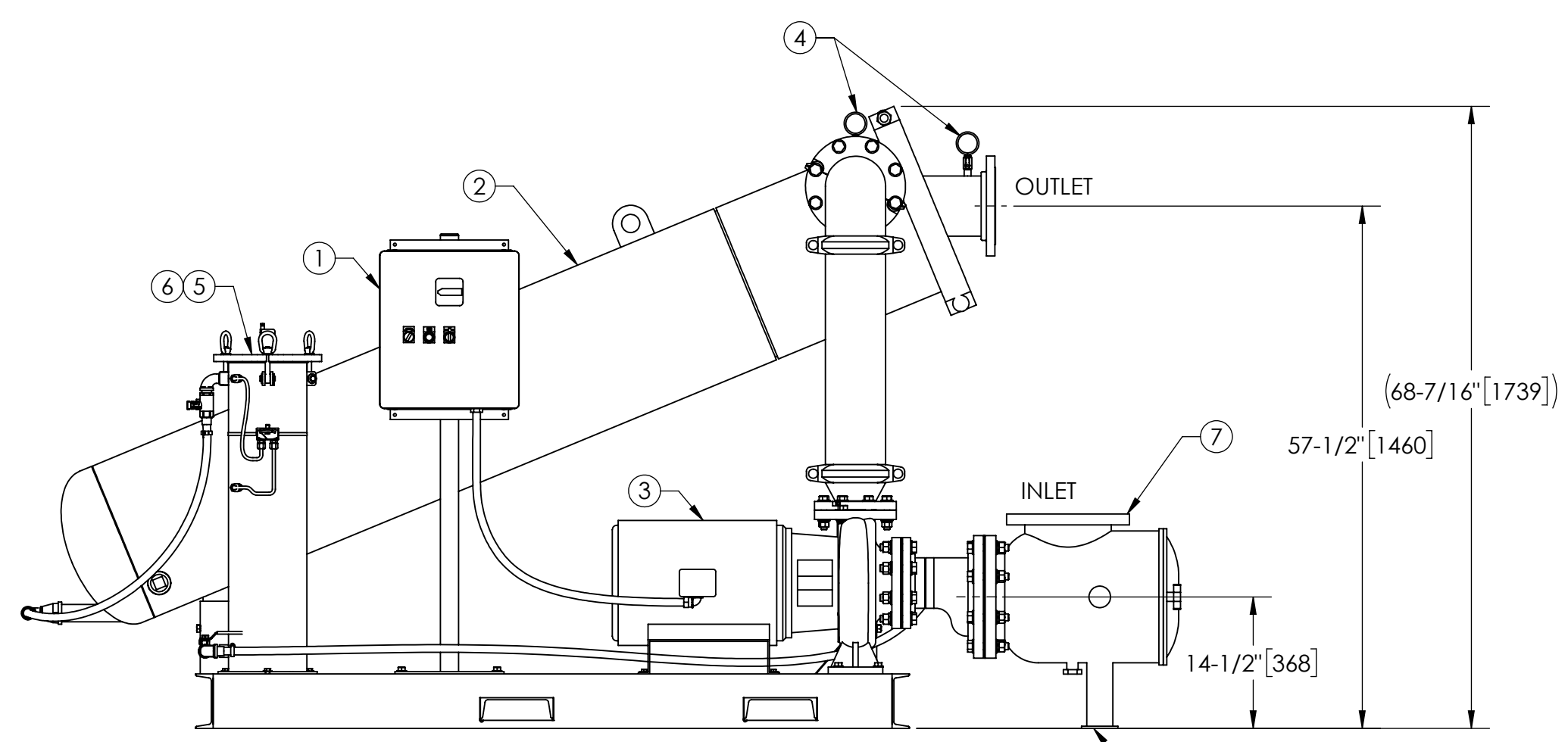
FRONT VIEW
