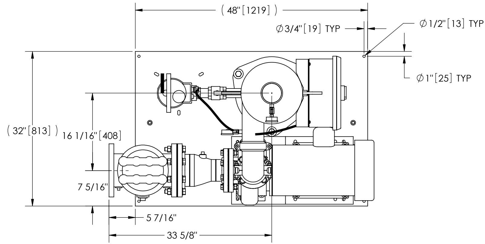
TOP VIEW
