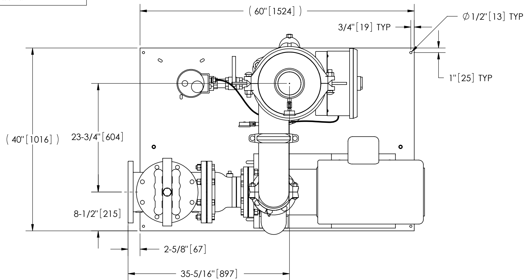
TOP VIEW
